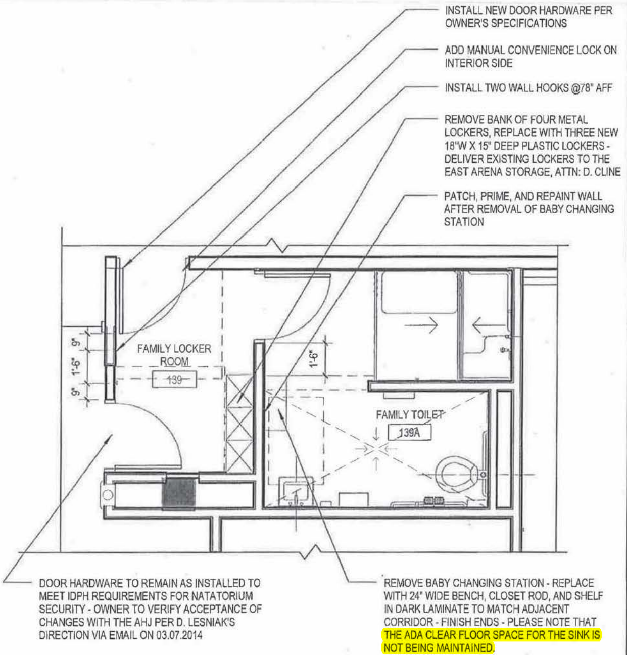
1 ENLARGED TOILET & LOCKER ROOM PLAN 1/4" = 1'-0"
